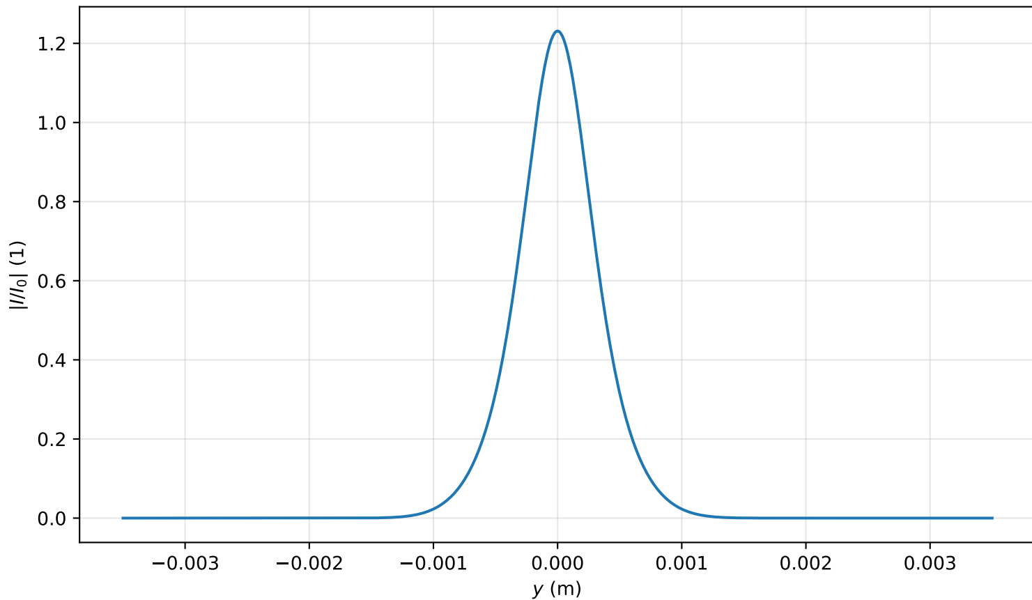
Intensity profile I(x=0, y, z=0.796)/I_0 , P_{in}=0.8P_{cr} , artificial time
